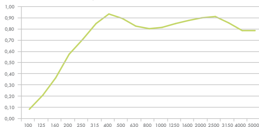
PICTURE ABSORBER, acoustic element wood-based sheet material 16 mm, acoustic perforation, wall distance 0 mm, acoustic dumping 50 mm Absorber class A \alpha_w 0.90 according to EN ISO 354
